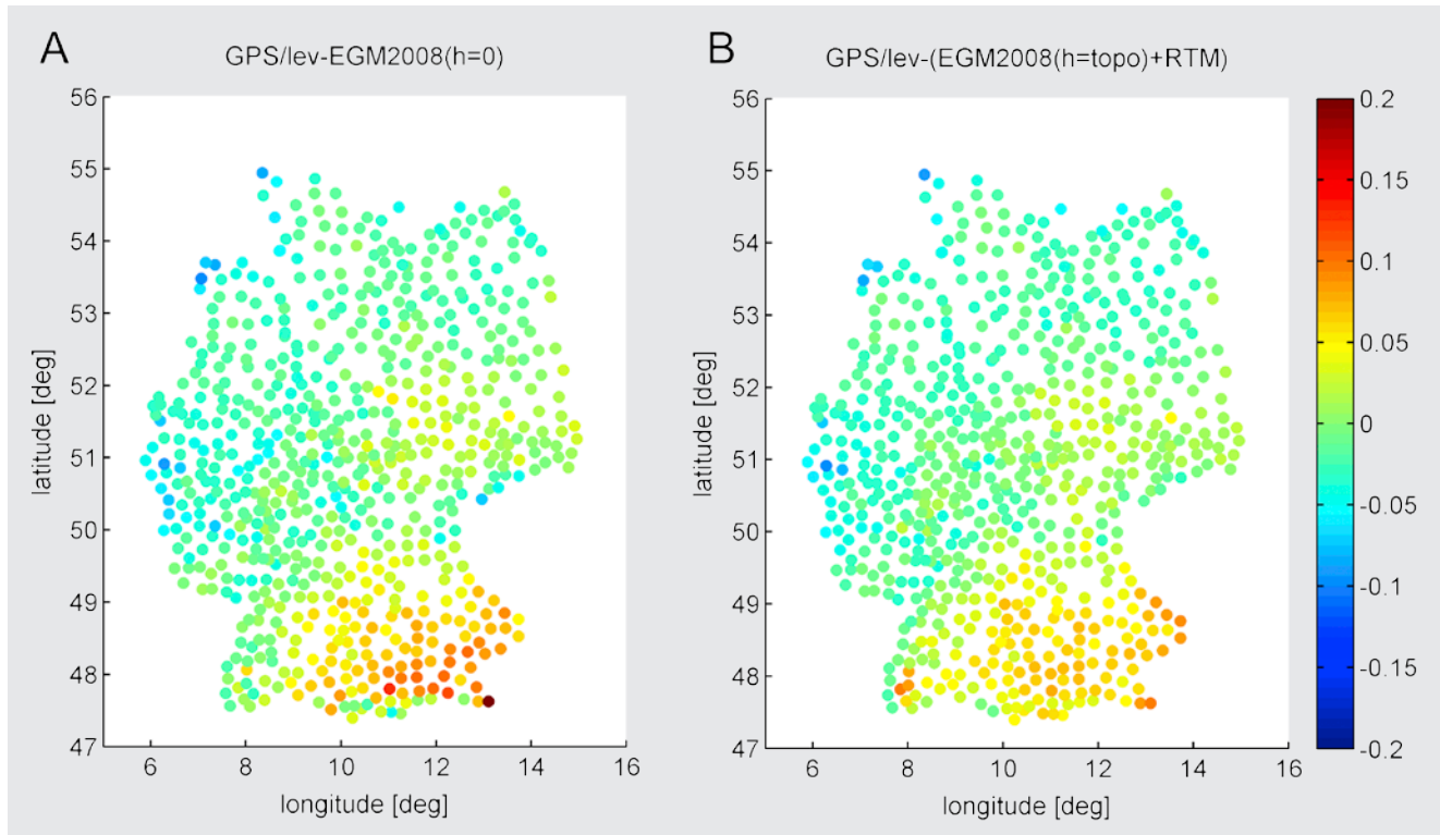
Fig. 8: Differences between GPS/levelling quasigeoid heights and variants of EGM2008. A: GPS/levelling – EGM2008 (evaluated on the ellipsoid), B: GPS/levelling – [EGM2008 (evaluated at the ellipsoidal height of the topography) + RTM]. Units in metres.
