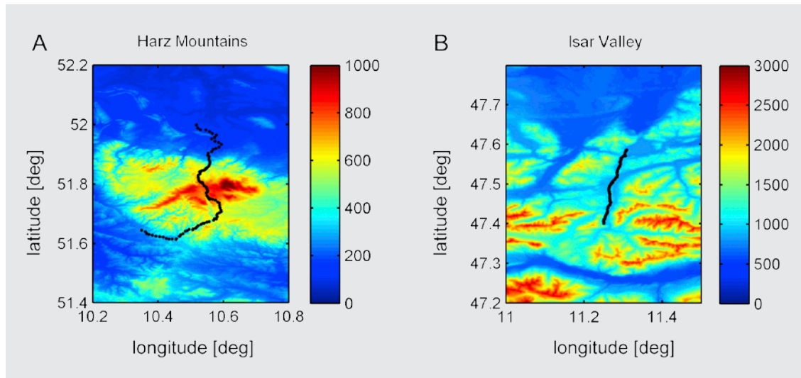
Fig. 6: Location of the astrogeodetic quasigeoid profiles. A: Harz Mountains profile, B: Isar Valley profile. The background topography are SRTM heights in metres.
