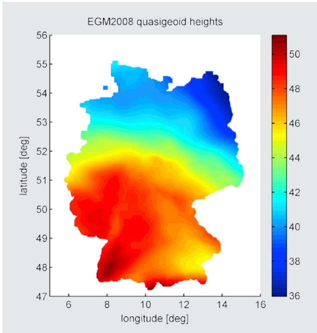
Fig. 1: EGM2008 quasigeoid heights over Germany (spectral degrees 2 to 2190, unit in metres)
