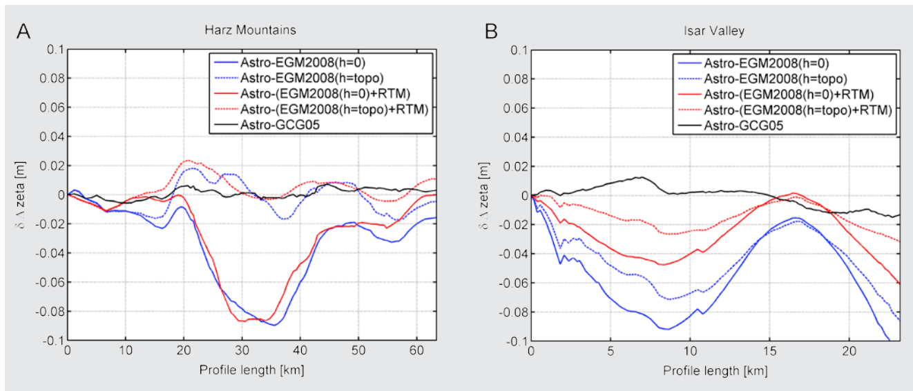
Fig. 9: Differences between the astrogeodetic quasigeoid heights and the EGM2008 variants (red, blue lines) and differences between the astrogeodetic quasigeoid heights and GCG05 (black lines). A: Harz Mountains, B: Isar Valley. The quasigeoid heights of the first profile points were set to zero for all data sets.
