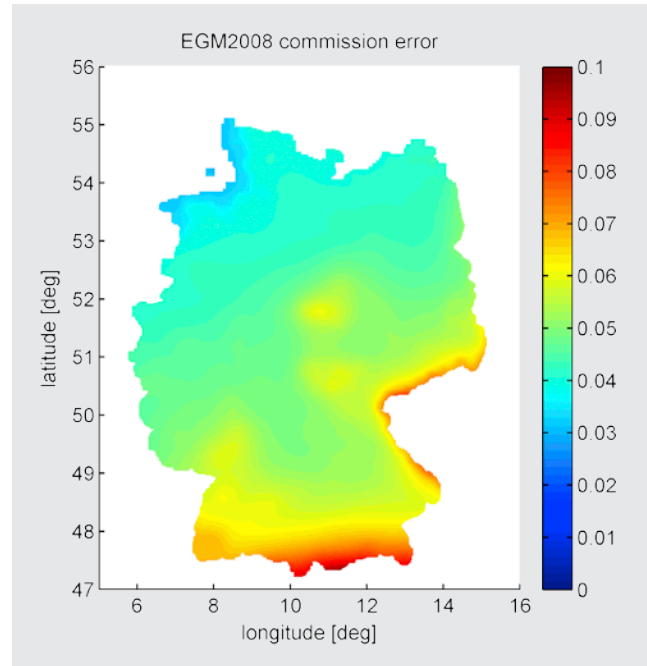
Fig. 2: EGM2008 commission errors over Germany (spectral degrees 2 to 2190, unit in metres)
