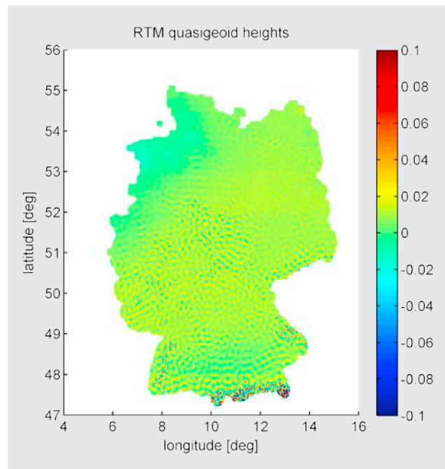
Fig. 4: RTM quasigeoid heights over Germany (unit in metres)
