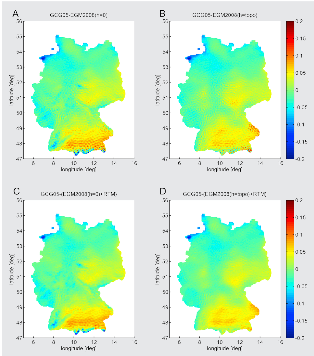
Fig. 7: Differences between the German Quasigeoid model GCG05 and variants of EGM2008. A: GCG05–EGM2008 (evaluated on the ellipsoid, h=0 ), B: GCG05–EGM2008 (evaluated at the ellipsoidal height of the topography), C: GCG05–[EGM2008 (evaluated on the ellipsoid, h=0 ) + RTM], D: GCG05–[EGM2008 (evaluated at the ellipsoidal height of the topography) + RTM]. Units in metres.
