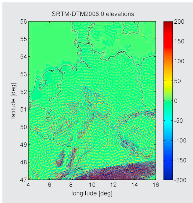
Fig. 3: RTM elevations (SRTM minus DTM2006.0) over Germany (unit in metres)
