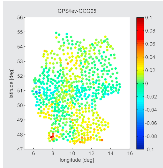
Fig. 5: Differences between quasigeoid heights of the 675 GPS/levelling points and GCG05 (unit in metres)
